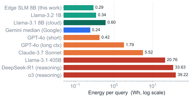
Fig. 2. Per-query inference energy (log scale). A sufficient SLM avoids the 3–65× energy of frontier/reasoning models [3], [4].
