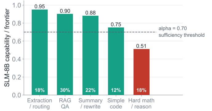
Fig. 3. Capability sufficiency by task class against the \alpha = 0.70 threshold. Green routes to the edge; red to cloud. The figure inside each bar is that class’s share of the workload. f_s = 82\% .
