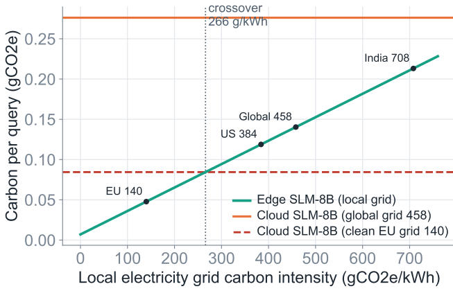
Fig. 5. Edge carbon scales with the local grid; it beats a clean cloud region only below the crossover intensity.
