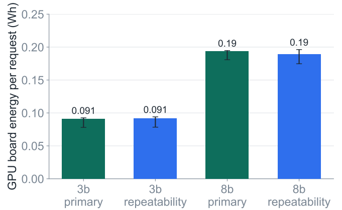
Fig. 11. Measured request-window GPU board energy on NVIDIA GeForce RTX 5070. Bars depict medians across seven repetitions; whiskers depict observed minima and maxima. Host platform draw, PSU losses, and post-request idle tails are evaluated via sensitivity analysis.
