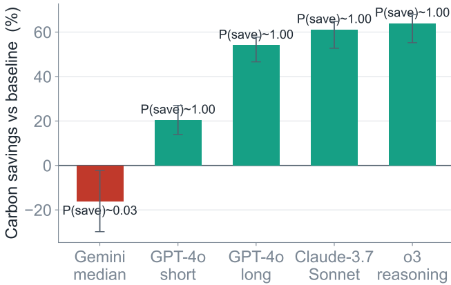
Fig. 6. Carbon savings (mean, 5–95% Monte-Carlo) vs. five cloud baselines. Positive only against frontier usage; refuted against best-in-class efficient cloud (Gemini, red).
