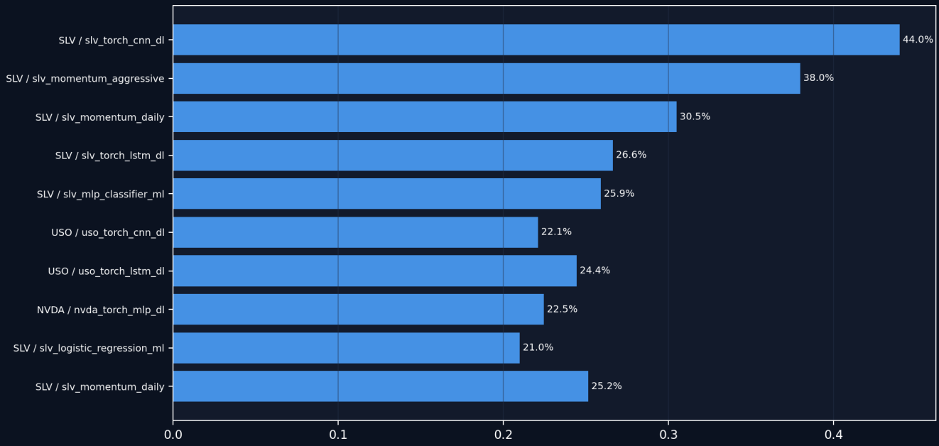
Top Strategies by Average Total Return
