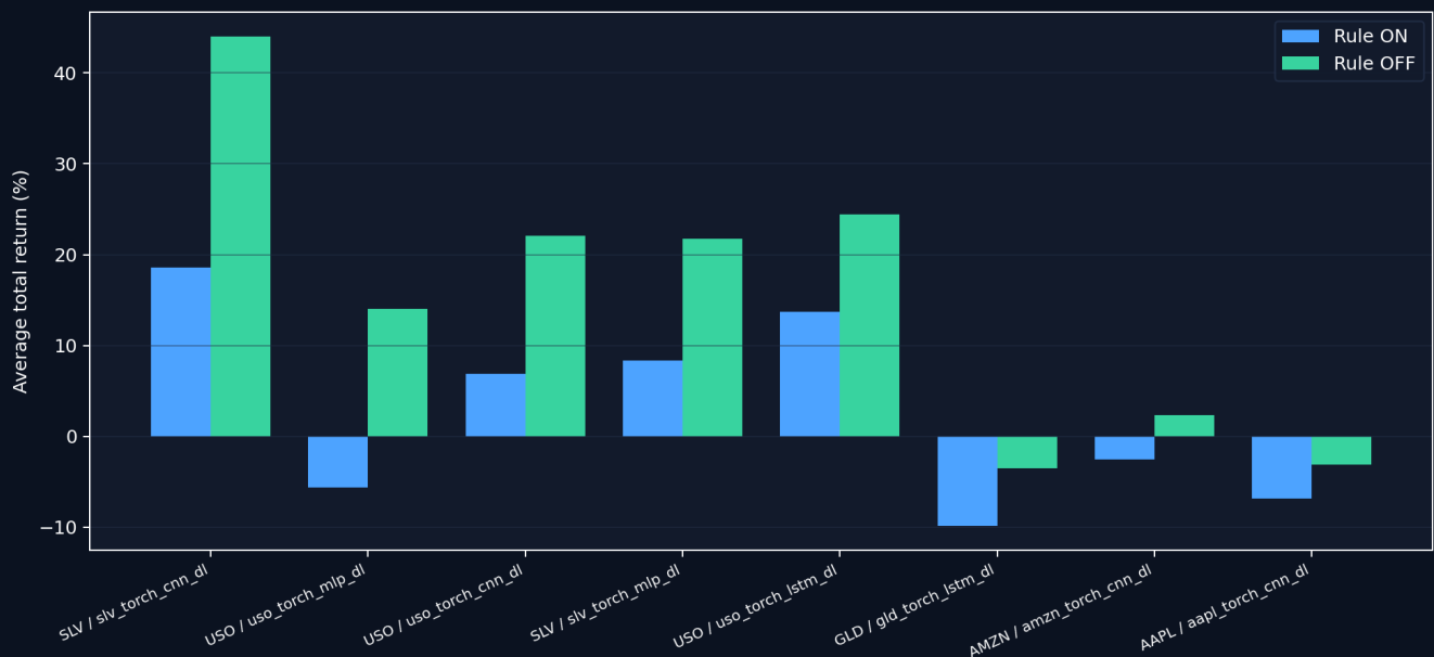
DL Average Total Return: No-Same-Day Reentry ON vs OFF
