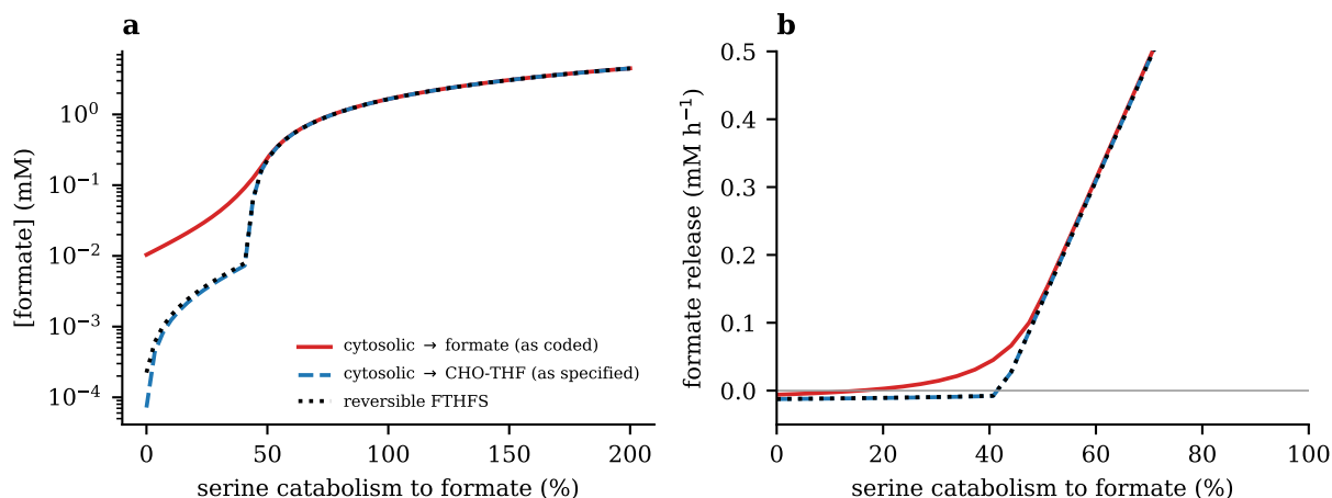
Figure 4: Cytosolic one-carbon routing (cyan condition, f_{S,CHO} = 0.5 ). (a) Intracellular formate; (b) formate release, the overflow threshold being the zero crossing. The reversible-FTHFS model (dotted) tracks the specified routing (dashed), not the coded one (solid).
