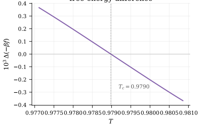
free-energy difference
