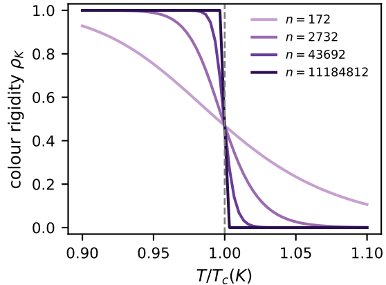
(a) K = 4 : the step is finite size
