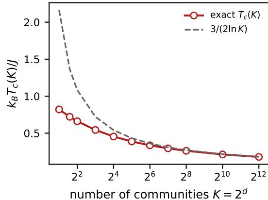
(c) T_c falls as the hierarchy deepens
