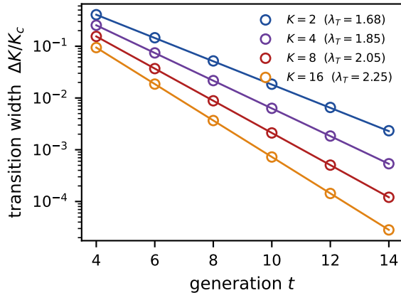
(b) width \sim \lambda_T^{-t} for every K
