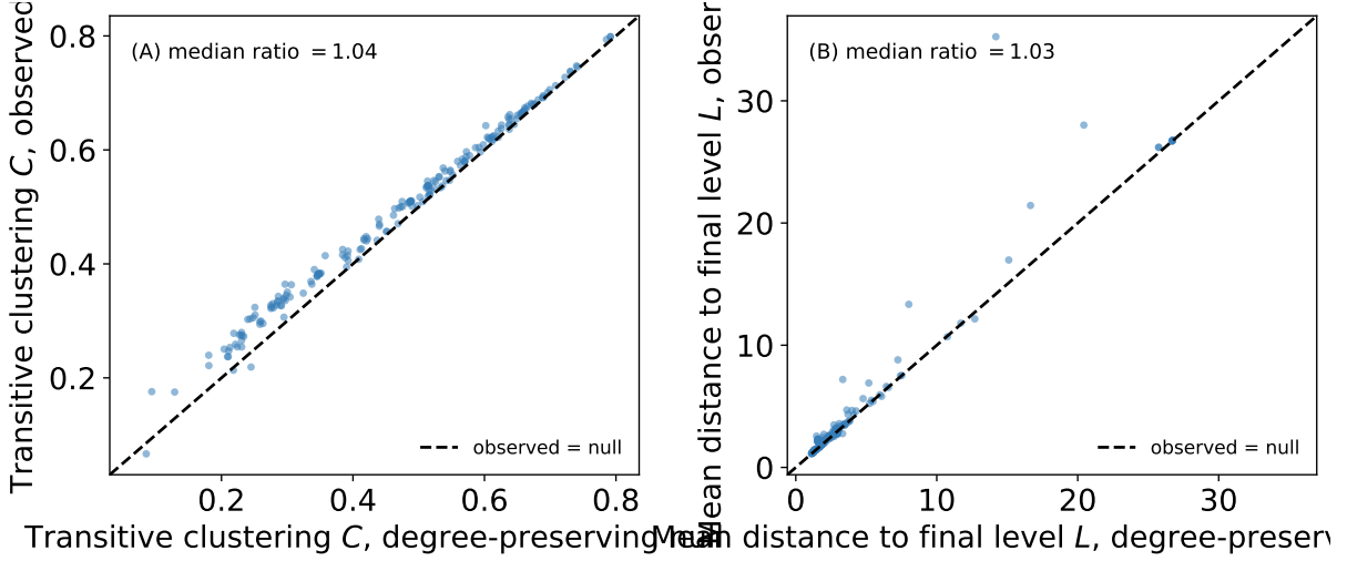
Figure 5: The shallowness follows from the degree distributions. Observed versus degree-preserving null values of (A) the transitive clustering coefficient C and (B) the mean distance to the final DUS level L , for 198 construction projects. The null holds the DUS spine fixed and rewires the skip dependencies while preserving every level’s skip in-degree and out-degree; each point is the average over 20 randomisations. Both quantities lie essentially on the identity line, so randomly reallocating the shortcuts reproduces what is observed.
