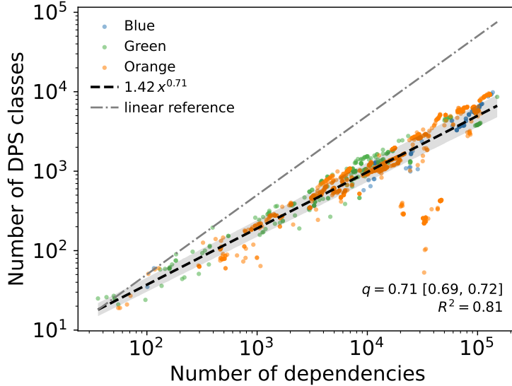
Figure 6: The number of DPS classes grows as a sub-linear power law with the number of dependencies. Each point is one of 1198 construction projects, coloured by company. The dashed line is the maximum-likelihood fit 1.42 x^{0.71} under multiplicative errors; the grey band is the 95% bootstrap confidence region. The dash-dotted line is a linear reference of slope 1.
