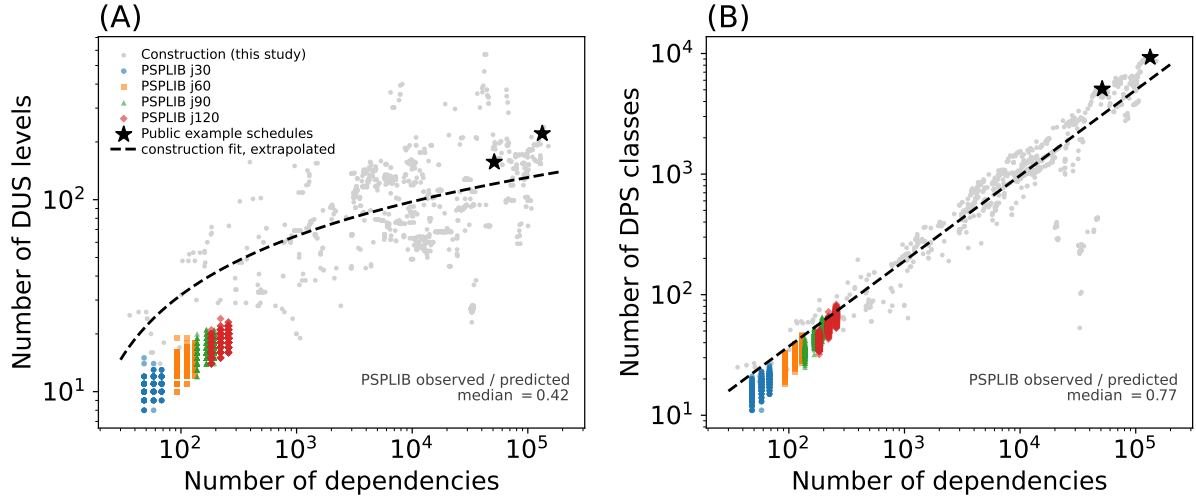
Figure 7: Replication on public benchmark instances. (A) Number of DUS levels and (B) number of DPS classes against the number of dependencies, for 2040 single-mode PSPLIB instances (coloured), the 1198 construction schedules of this study (grey), and the two anonymised real schedules distributed with the code repository (stars). Dashed lines are the fits to the construction data, evaluated two orders of magnitude below the median project size on which they were estimated. Only 2.4% of the construction projects are as small as the largest PSPLIB instance.
