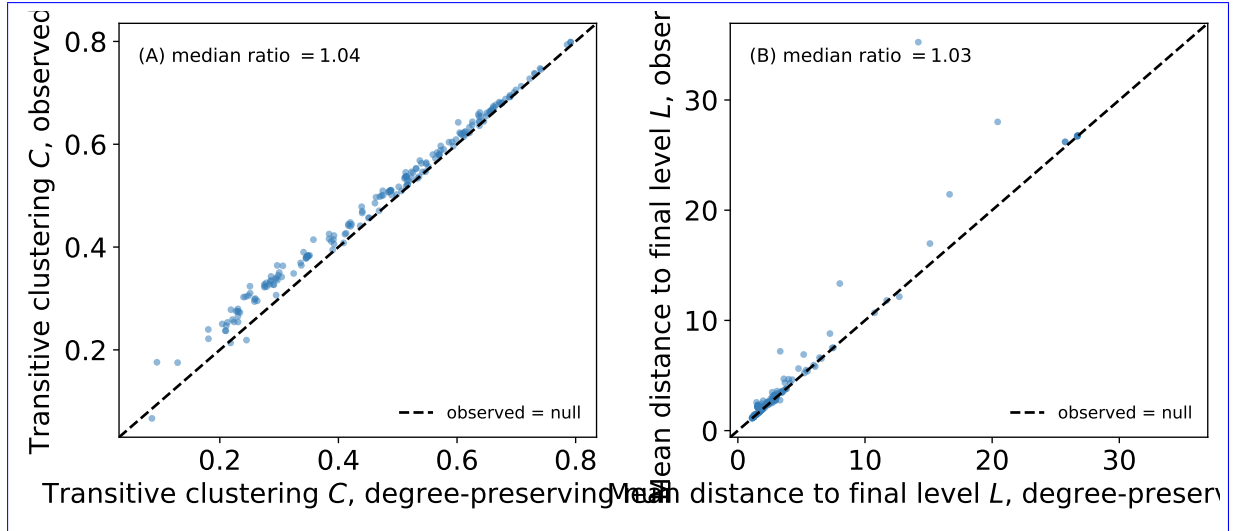
Figure 5: The shallowness follows from the degree distributions. Observed versus degree-preserving null values of (A) the transitive clustering coefficient C and (B) the mean distance to the final DUS level L , for 198 construction projects. The null holds the DUS spine fixed and rewires the skip dependencies while preserving every level’s skip in-degree and out-degree; each point is the average over 20 randomisations. Both quantities lie essentially on the identity line, so randomly reallocating the shortcuts reproduces what is observed.
