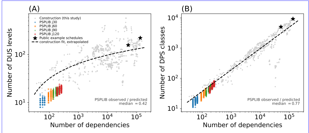
Figure 7: Replication on public benchmark instances. (A) Number of DUS levels and (B) number of DPS classes against the number of dependencies , for 2040 single-mode PSPLIB instances (coloured), the 1198 construction schedules of this study (grey), and the two anonymised real schedules distributed with the code repository (stars). Dashed lines are the fits to the construction data, evaluated two orders of magnitude below the median project size on which they were estimated. Only 2.4% of the construction projects are as small as the largest PSPLIB instance.
