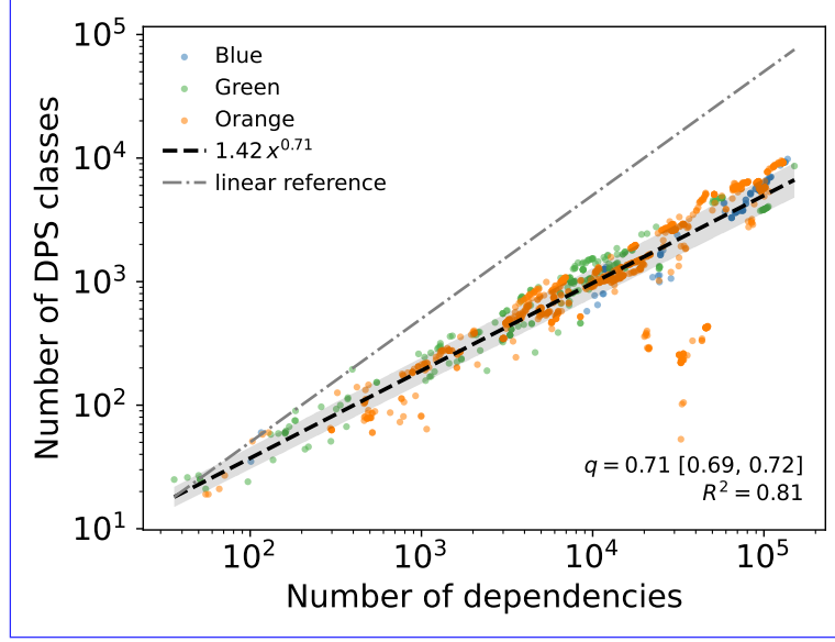
Figure 6: Nodes in The number of DPS classes grows as a dependency network are stratified based on their dependency patterns. Node colour indicates sub-linear power law with the DFS number of dependencies. Each point is one of 1198 construction projects, and coloured by company. The dashed line is the node label gives maximum-likelihood fit 1.42x^{0.71} under multiplicative errors; the DUS grey band is the 95% bootstrap confidence region. The dash-dotted line is a linear reference of slope 1.
