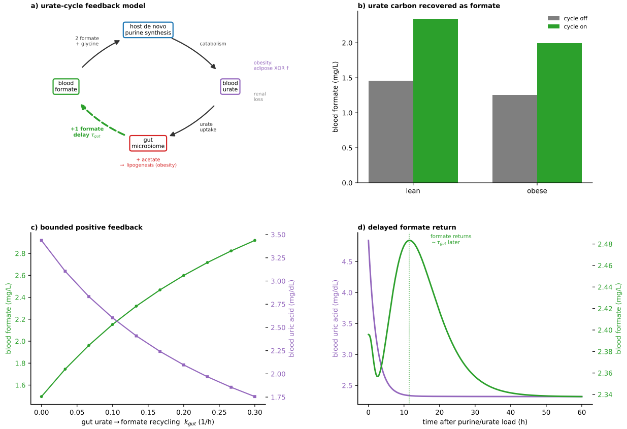
Figure 8: The gut microbiome closes a urate cycle: a delayed positive feedback. A gut-microbiome compartment degrades blood urate and returns formate after a delay \tau_{gut} . (a) Schematic of the model: host purine synthesis consumes two formate (plus glycine) per urate; the gut microbiome returns one of them as formate after the delay \tau_{gut} (green, closing the loop) and co-produces acetate ( \rightarrow lipogenesis). (b) Steady-state blood formate with the cycle off versus on, lean and obese — urate carbon is recovered as formate. (c) As the gut urate \rightarrow formate recycling k_{gut} strengthens, blood formate rises and blood urate falls, both converging: a bounded positive feedback (loop gain < 1 ). (d) A purine/urate load clears from the blood within hours but returns as a blood-formate rise \sim \tau_{gut} ( \sim 12 h) later.
