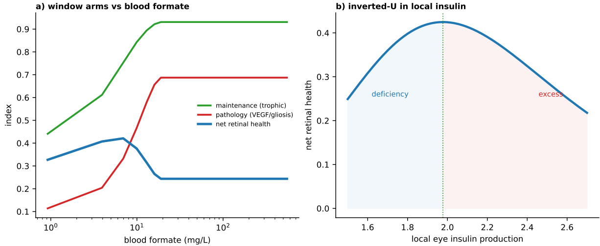
Figure 14: Retinal health is an optimal window in local insulin. Retinal health is scored as a trophic maintenance arm minus a higher-threshold pathology arm (VEGF/gliosis/neovascularization); no complex-IV inhibition is invoked. (a) across blood formate, maintenance, pathology and net health (markers at 5, 50, 500 mg/L); (b) net health is an inverted-U in local eye insulin — both deficiency (low formate) and excess (high formate) harm the retina.
