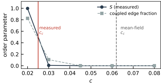
(b) converged transition vs mean field
