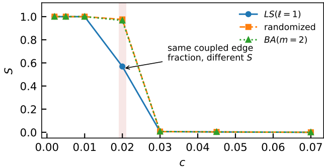
(a) local structure fragments the coupled phase
