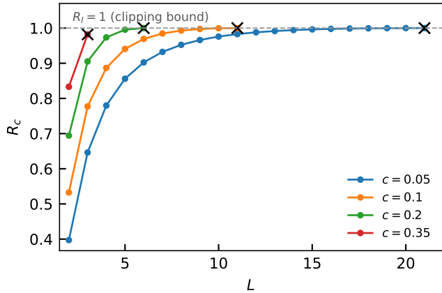
(b) critical line; \times marks a = 1/c
