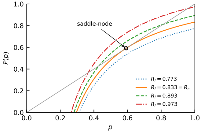
(a) return map, L = 2 , c = 0.35
