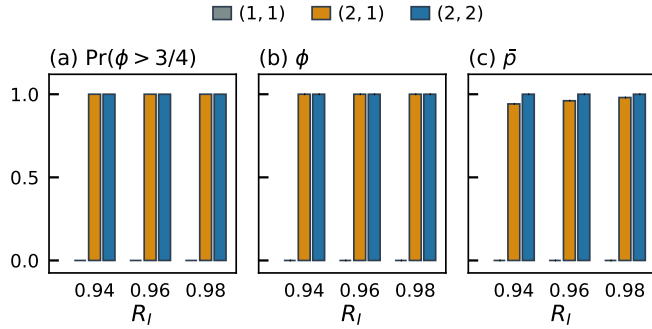
FIG. 3. Asymmetric pairing at L = 3 , \tau_{\text{mem}} = 50 , \epsilon = 0 , 2 \times 10^5 steps, N = 40 independent realisations per bar. Bars are grouped by the value R_I of the interaction and, within a group, by the modelling levels ( A, B ) of the two agents. A single level-2 agent holds the pair in the coupled phase. (a) Fraction of realisations ending coupled, \phi > 3/4 ; (b) occupancy \phi ; (c) time-averaged participation propensity \bar{p} . The axis runs a little below zero so that a bar of height zero still shows its outline: the level-1 pairs (1, 1) collapse in every realisation, at every R_I . The outcome is otherwise deterministic, all 40 realisations agreeing, so the error bars are invisible except on \bar{p} — and \bar{p} is the only thing promoting the second agent changes, which is the content of the (2, 1) against (2, 2) comparison. The column headed “occupancy” in the corresponding table of the first submission was in fact \bar{p} ; the two are shown separately here.
