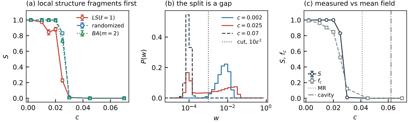
FIG. 5. Percolation of the solitary phase. All panels: n = 600 , \langle k \rangle = 4 , R_I = 0.95 , 4 \times 10^5 steps, N = 24 independent realisations per point, error bars the standard error over realisations. (a) Giant component S of the coupled subgraph against the cost c of an unreciprocated offer. At c = 0.025 the three rules carry the same coupled edge fraction f_c , to within 0.006, but only the local rule fragments. (b) Distribution P(w) of the per-edge interaction rate w , pooled over realisations of LS(l = 1) . A collapsed edge executes only when both endpoints explore, which places it near 10^{-4} ; a coupled edge executes two orders of magnitude more often. The classification cut 10\epsilon^2 , dotted, lies in the gap between the two bands. (c) Coupled edge fraction f_c and S on the randomized network, with the two mean-field thresholds marked, Molloy-Reed (MR, dotted) and cavity (dash-dotted): the transition lies between c = 0.025 and c = 0.030 , against c_c = 0.041 from Eq. (9) and c_c = 0.062 from Eq. (10). (b) Converged runs ( 4 \times 10^5 steps) place the transition between c = 0.020 and c = 0.030 ; Eq. (10) predicts c_c \simeq 0.062 .
