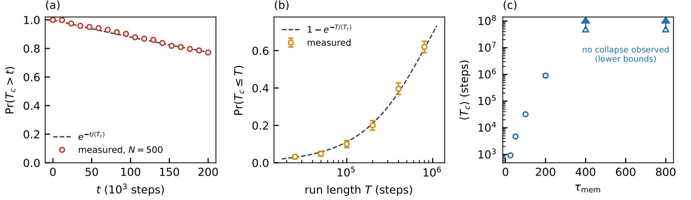
FIG. 4. Escape from the coupled state is a rare event with a constant hazard. Reference point L = 2 , c = 0.35 , R_I = 0.8428 , \epsilon = 10^{-2} , \tau_{\text{mem}} = 200 . Symbols are measurements throughout; dashed lines are the exponential law with \langle T_c \rangle taken from the censored maximum likelihood. (a) Probability that the collapse time exceeds t , over N = 500 independent realisations. (b) Probability that it does not exceed the run length, against that run length, N = 250 per point, compared with the single rate pooled over all six lengths; error bars are binomial. (c) Mean collapse time against the memory time, N = 250 per point; open triangles are lower bounds at \tau_{\text{mem}} = 400 and 800 , where no realisation collapsed.
