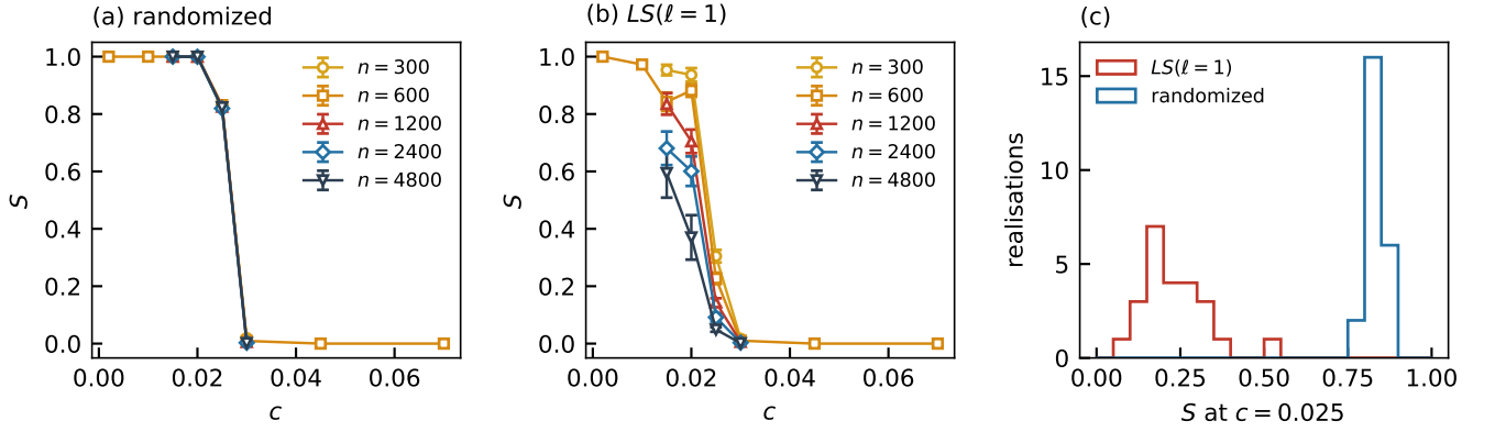
FIG. 6. The network transition with system size. (a) Giant component of the coupled subgraph against c on the randomized network at five sizes; (b) the same for triadic closure, LS(\ell = 1) ; (c) distribution of S over the N = 24 realisations at c = 0.025 , n = 600 , where the two rules differ most. Error bars in (a) and (b) are standard errors over realisations, N as in Supp. Tab. IV.
