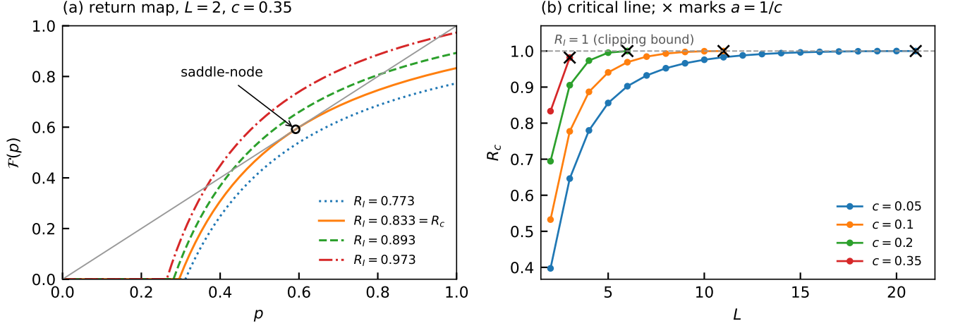
FIG. 1. (a) Return map \mathcal{F}(p) for L = 2 , c = 0.35 at several R_I , with the diagonal in grey. The two nontrivial fixed points are born in a saddle-node at R_c = 0.8332 , p^* = 0.5916 (circle). (b) Critical line R_c(L) from Eq. (6) for several costs c ; crosses mark the validity boundary a = 1/c , Eq. (7), beyond which no interior bifurcation exists.
