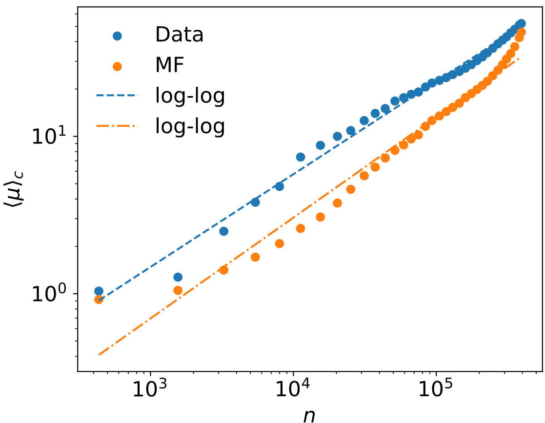
c) arxiv/cond-mat co-authorship
