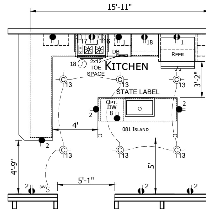
OPTIONAL ULTIMATE KITCHEN 2
