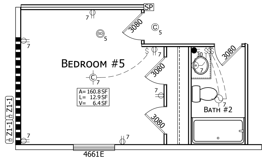
OPTIONAL 5TH BEDROOM
