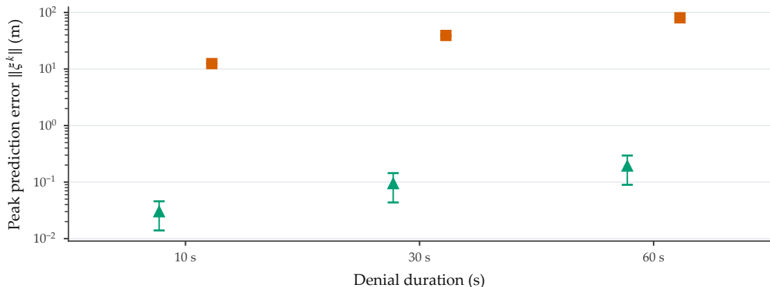
(c) Prediction error \|\xi^k\| keeps growing
