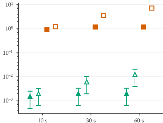
(c) Prediction error \|\xi^k\| keeps growing
