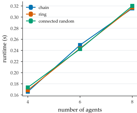
(b) wall-clock cost
