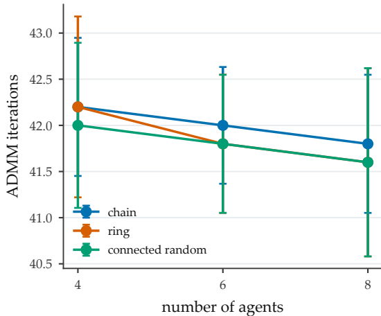
(a) iteration cost
