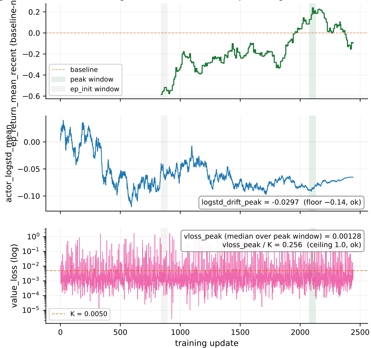
Fig 20 — SIG-EXPLORATION signature on seed 9 (CTS-reproducing in both measurement passes)
