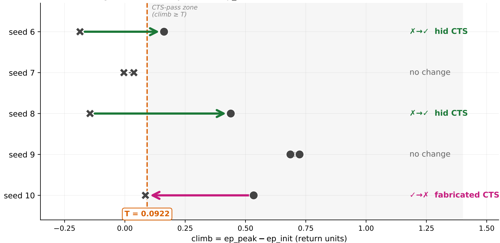
Fig 3 — Direction-symmetric ep_init-window confounder on seeds {6..10} (KEY)
