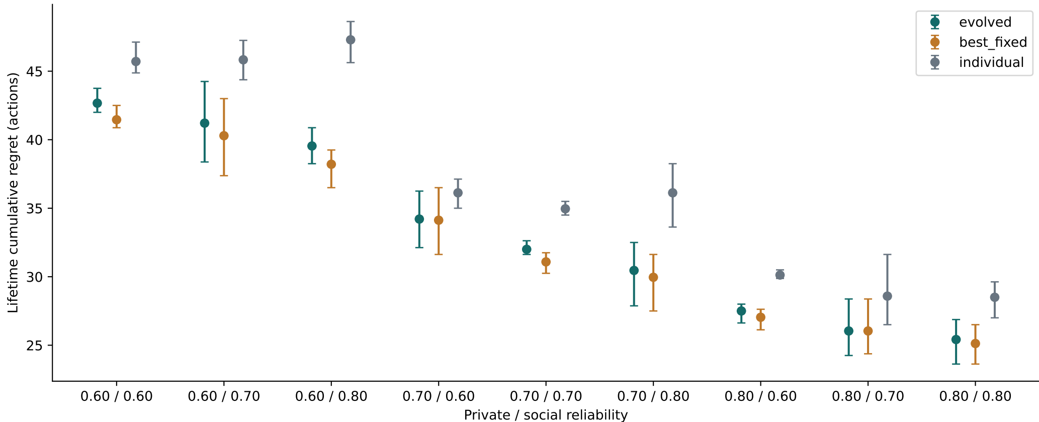
Generalization across unseen reliability pairs
