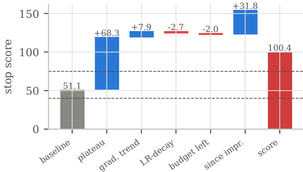
lr0.001_bs64_s0, after epoch 34: early_stop
