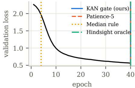
lr=0.0001, batch=256
