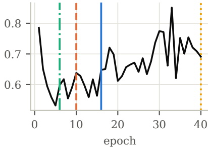
lr=0.03, batch=64
