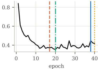
lr=0.001, batch=64
