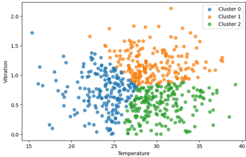
KMeans Clusters (k=3)
