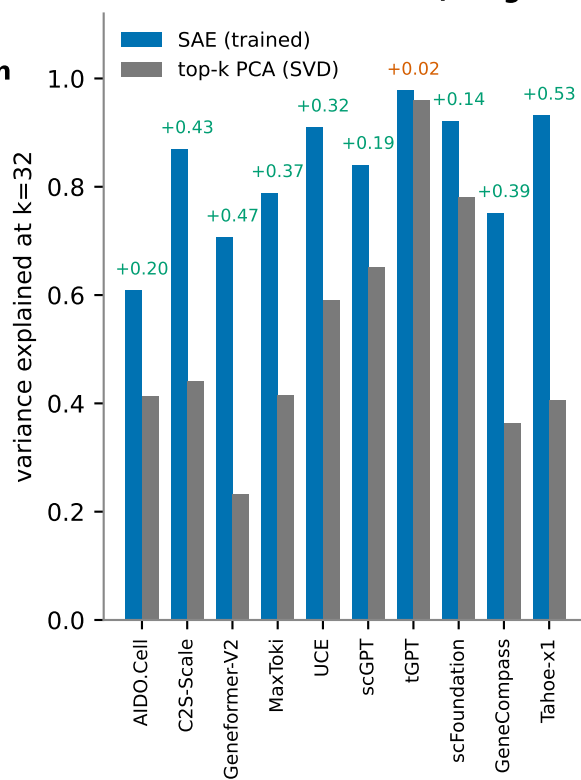
B SAE > PCA in all ten (margin varies)
