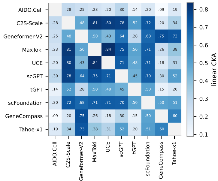
A Cross-model geometry — CKA, 50% depth
