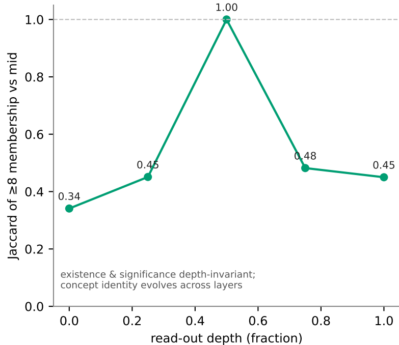
Fig S2 The shared backbone is robust to layer choice (a depth-invariant phenomenon, mid-depth-specific membership)
