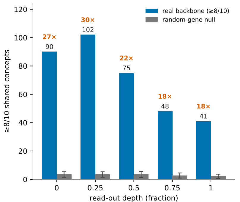
Fig S2 The shared backbone is robust to layer choice (a depth-invariant phenomenon, mid-depth-specific membership)
