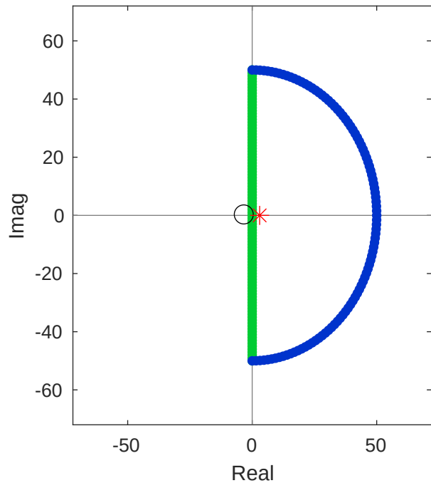
PZMAP + CONTOUR (poles red, zeros black)
