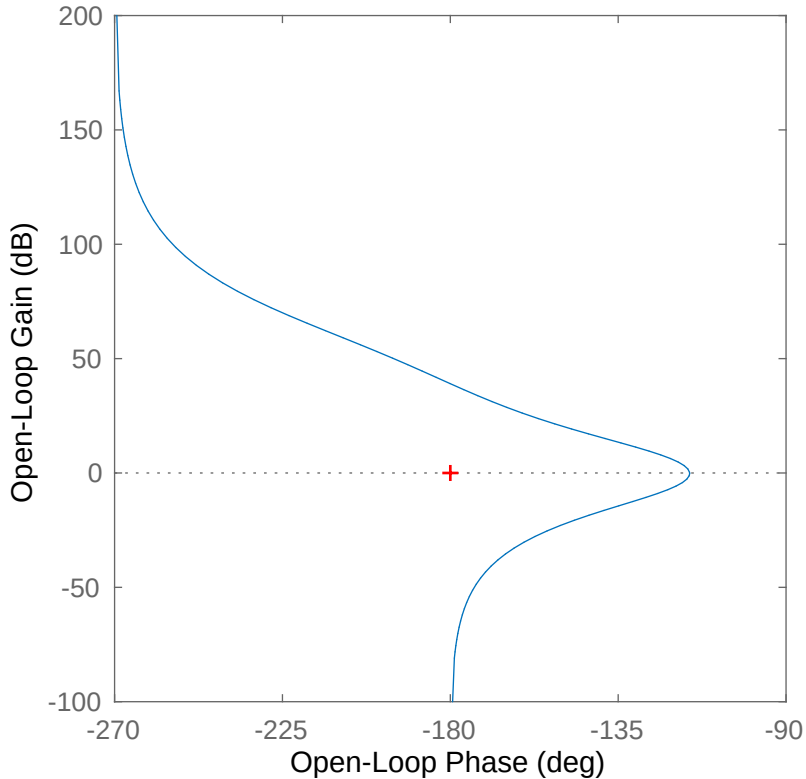
Nichols Chart
