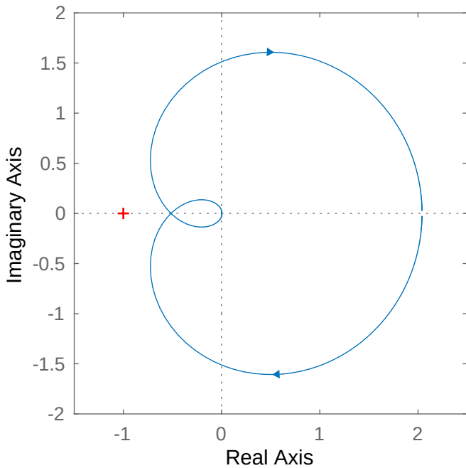
Nyquist Diagram
