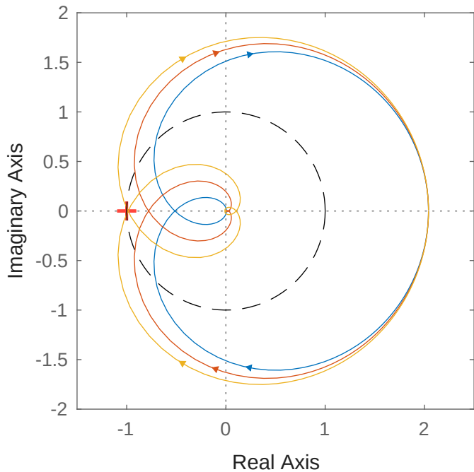
Nyquist Diagram
