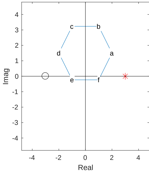
PZMAP + CONTOUR (poles red, zeros black)
