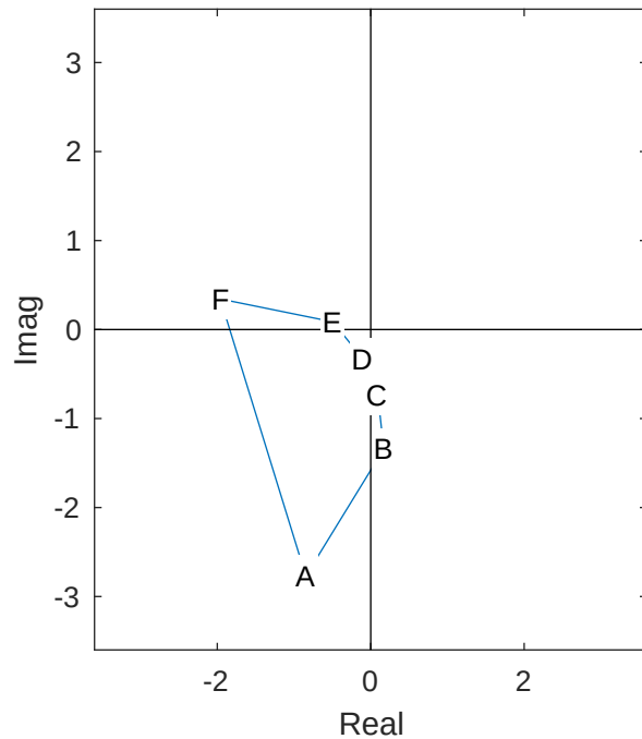
CONTOUR MAPPED THROUGH G(s) (e.g., A = G(a) , B = G(b) , etc.)
