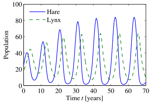
(a) Time response
