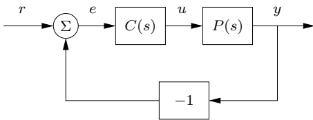
(a) Closed loop system
