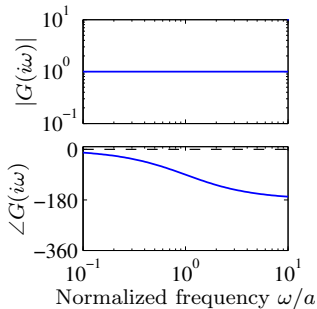
(b) Right half-plane zero
