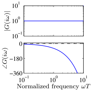
(a) Time delay
