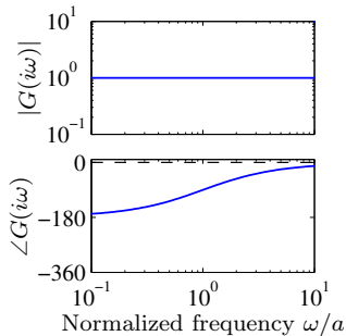
(c) Right half-plane pole
