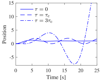
(b) Closed loop step responses
