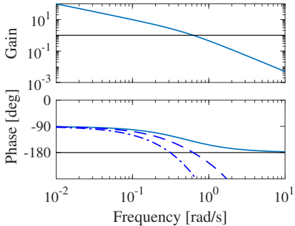
(a) Loop transfer function
