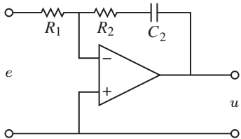
(a) PI controller
