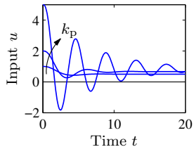
(a) Proportional control
