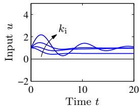
(b) PI control
