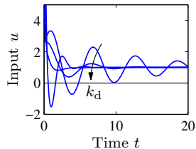
(c) PID control
