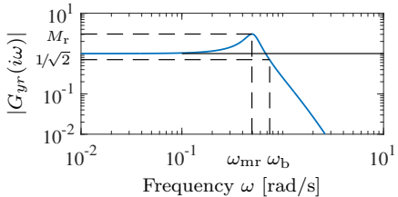
(b) Frequency response of G_{yr}(i\omega)
