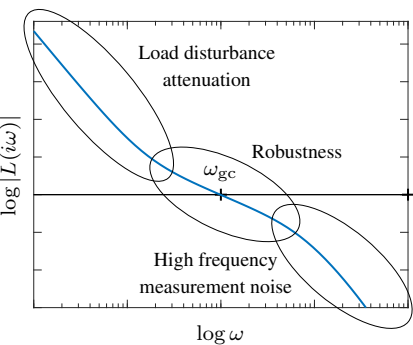
(a) Gain plot of loop transfer function
