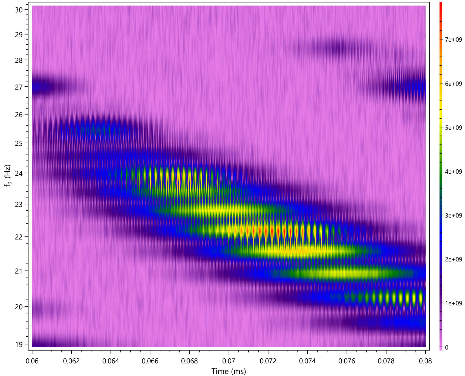
complexTransientModulus Plot
