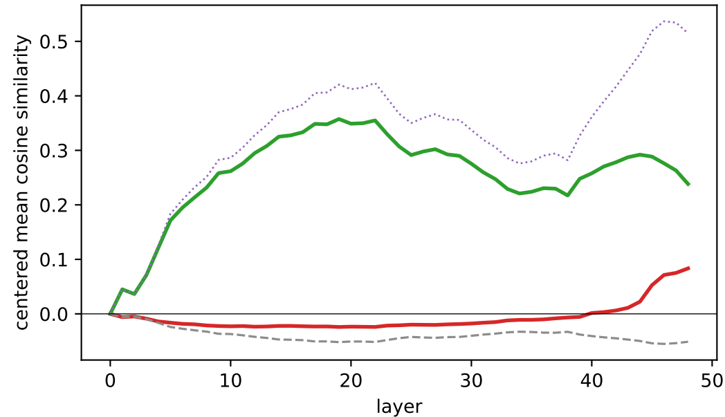
EVA-CLIP-18B (language-supervised)
