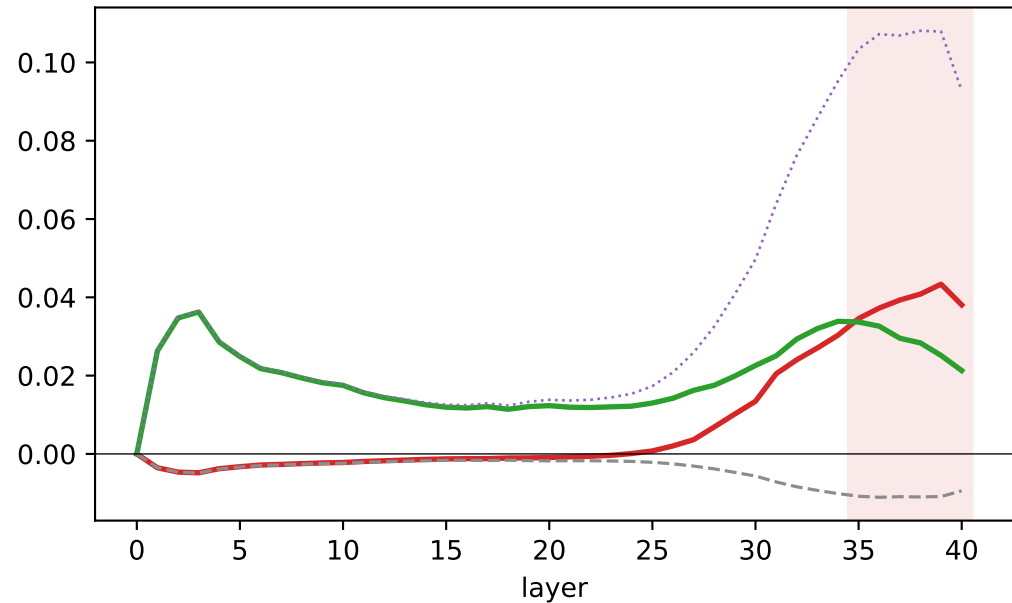
DINOv3-7B (self-supervised)
