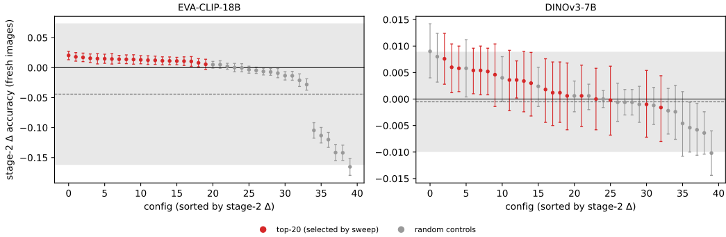
Figure 5: Stage-two confirmation on fresh images. Each point is a configuration’s across-dataset mean \Delta accuracy on 500 held-out images per dataset (bars: 95% paired-bootstrap CIs); red = top-20 from the sweep, gray = random controls; shaded band = \mu_{\text{ctrl}} \pm 2\sigma_{\text{ctrl}} . In both models the selected configurations replicate small positive effects (CIs above zero) but none clears the pre-specified control band (Eq. 1).
