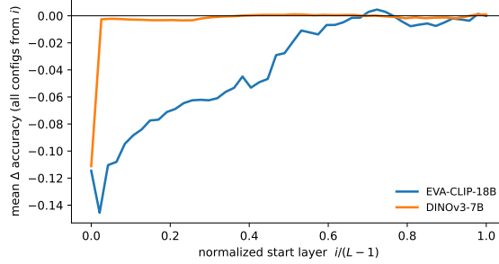
Figure 3: Depth profile of duplication damage. Mean random-split \Delta accuracy of all configurations starting at layer i , averaged over datasets, against normalized depth. Both models converge to zero damage as the duplicated region moves toward the output—the reverse of the LLM profile, where late-layer duplication is catastrophic. DINOv3-7B is uniformly more tolerant.
