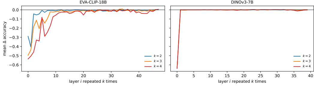
Figure 6: Single-layer repetition (exploratory; no confirmation stage). Mean random-split \Delta accuracy over datasets when layer i is executed k times. Early-layer damage compounds with k in EVA-CLIP-18B (regional mean -22 pp at k=3 , -35 pp at k=4 ) but saturates in DINOv3-7B; mid- and late-stack repetition remains near-free in both models even at k=4 .
