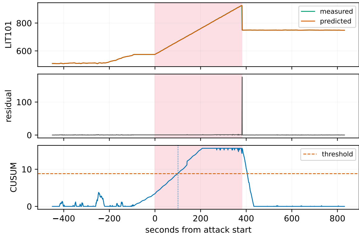
SWaT attack 3 alert
