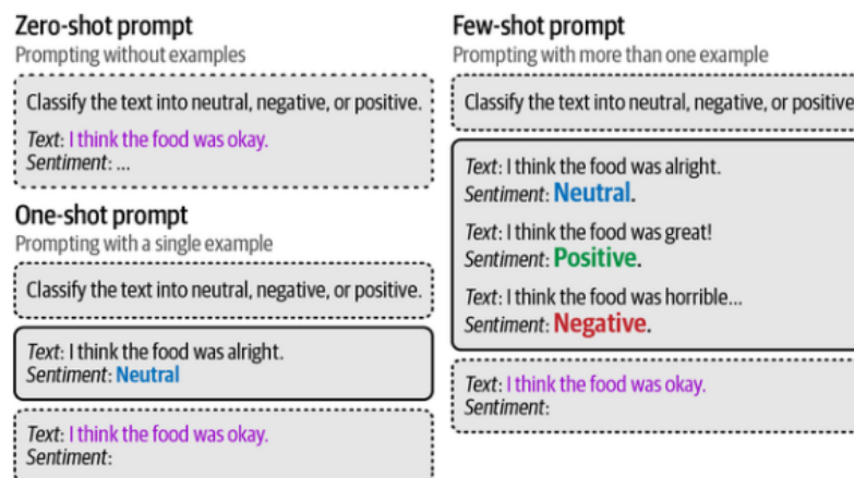
Figura 2.25: Representaciones de zero-shot, one-shot y few-shot
