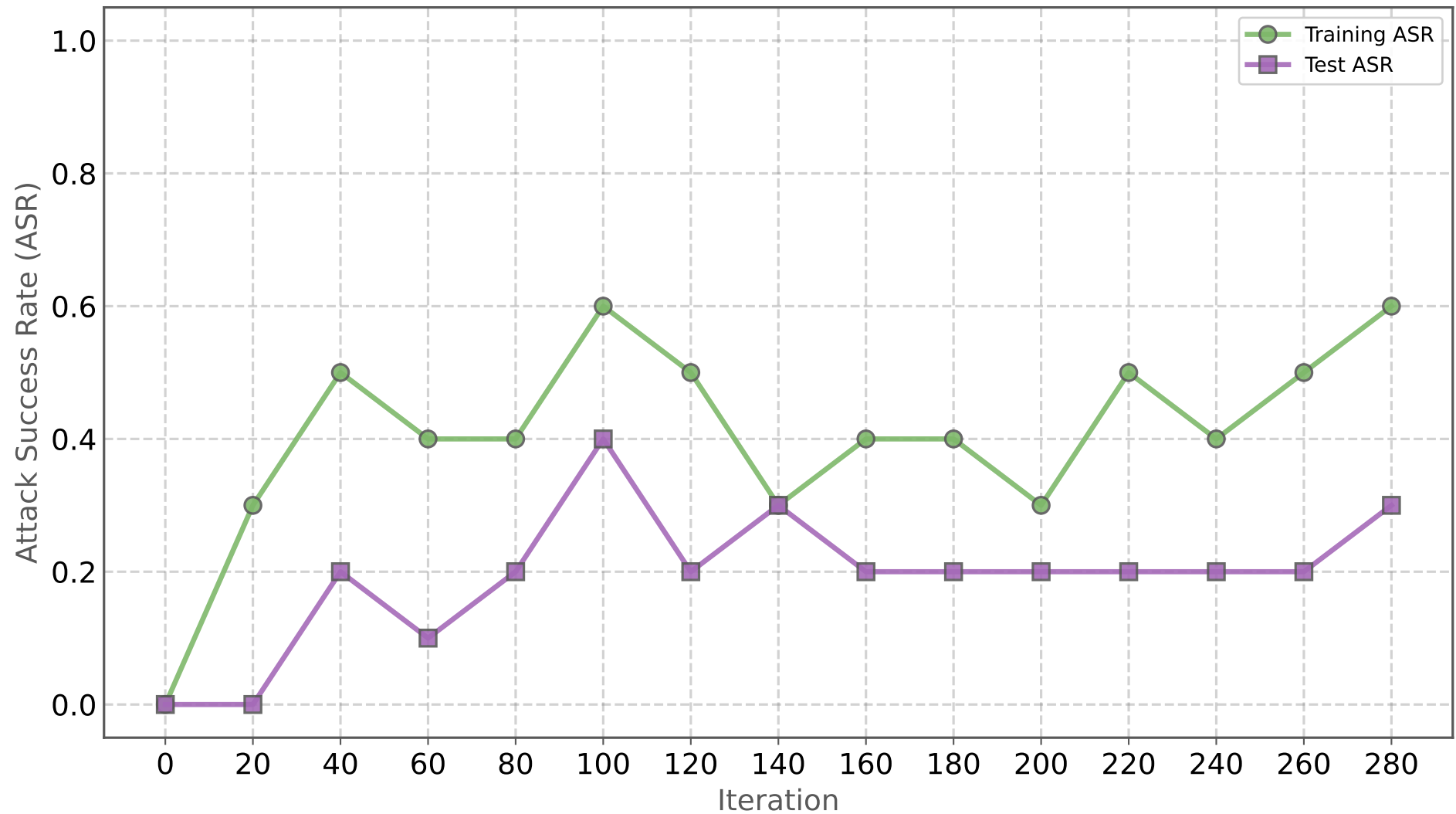
Universal GCG: ASR Over Iterations
