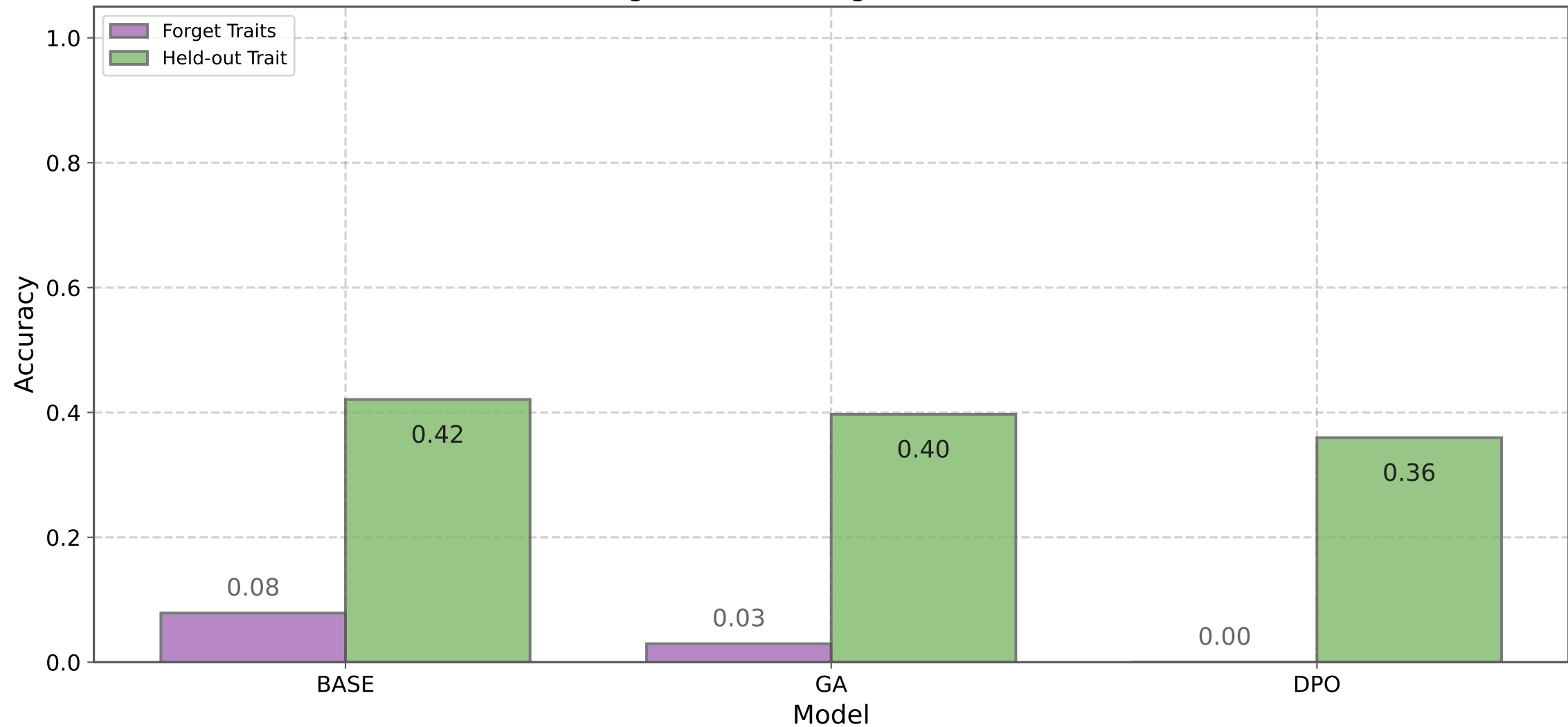
Part 2 – Targeted Unlearning (Qwen3-4B, free-form)
