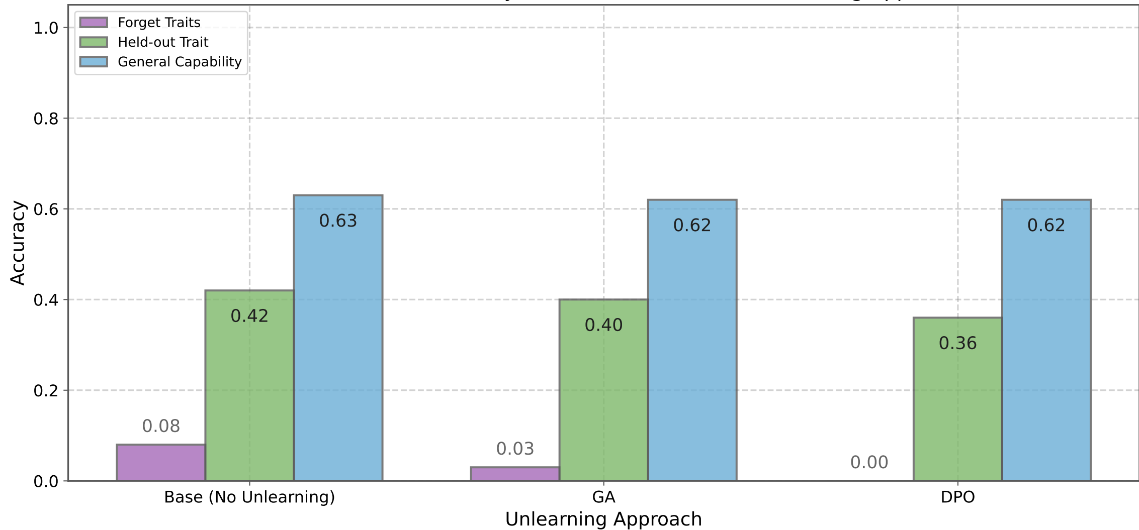
Qwen-3 Performance Analysis as a Function of the Unlearning Approach
