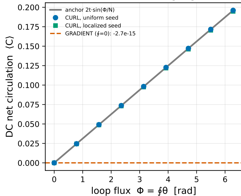
Discriminator: curl drives, gauge does not
