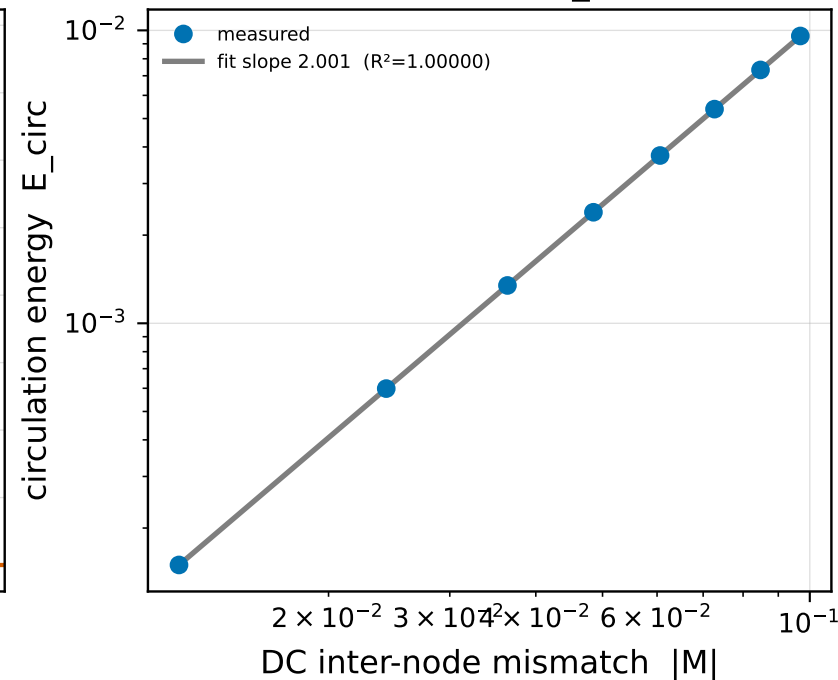
Mass observable: E_{\text{circ}} \propto M^2
