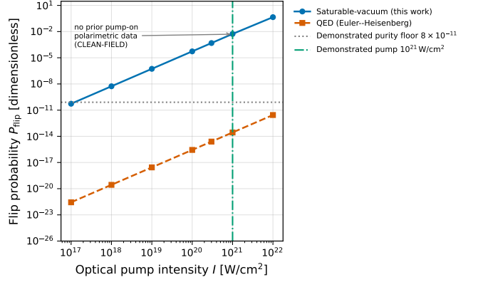
FIG. 1. The exposure plane. Predicted polarization-flip probability P_{\text{flip}} versus optical-pump intensity for the saturable-vacuum model (blue, Eqs. (3) and (9)) and for the QED Euler–Heisenberg co-prediction (orange, Eq. (8)), through the identical single-pass readout chain at probe energy 9835 eV, z = 10 \mu\text{m} . Both scale as intensity squared, so their ratio is field-independent. The dotted line marks the record X-ray-polarimeter purity ( 8 \times 10^{-11} , Ref. [12]; the conservative 2.4 \times 10^{-10} single-measurement floor of Ref. [13] used for the kill criterion lies just above it), and the dash-dot line the demonstrated ReLaX pump ( 10^{21} \text{ W cm}^{-2} ). No prior experiment occupies the pump-on polarimetric exposure region, so the model’s prediction there is unconstrained by existing data.
