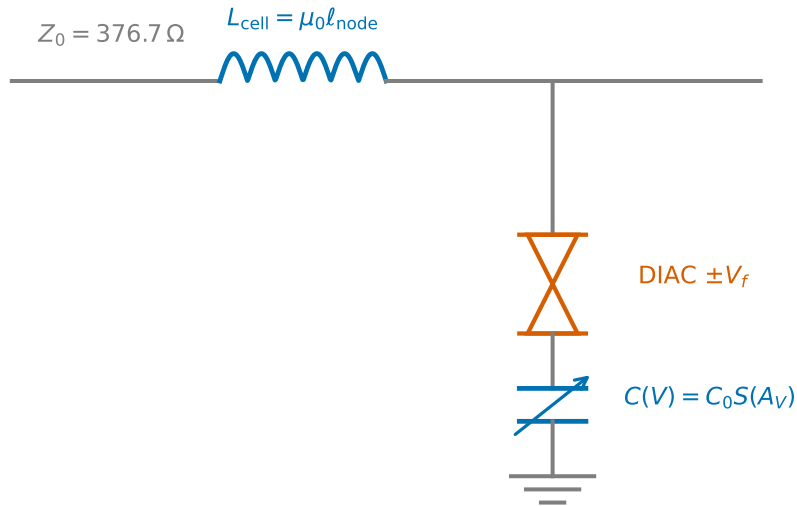
lossless LC link + DIAC-gated T2 varactor (one cell)
