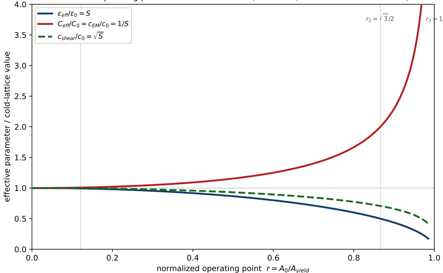
Substrate operating-point characteristic curves (Vol 9 Ch 7, Table of saturation curves)
